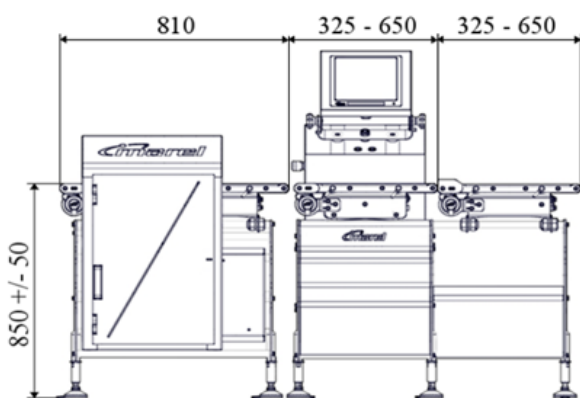
Standard weigh table with infeed and single reject shown.
